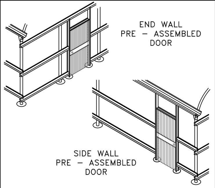
1 PRE - ASSEMBLED DOOR
