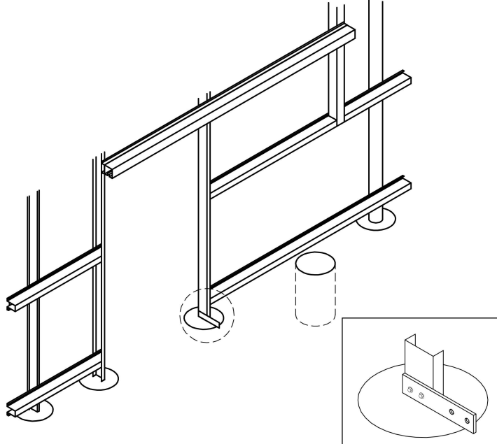
1 BOTTOM TRACK FLAT BAR
