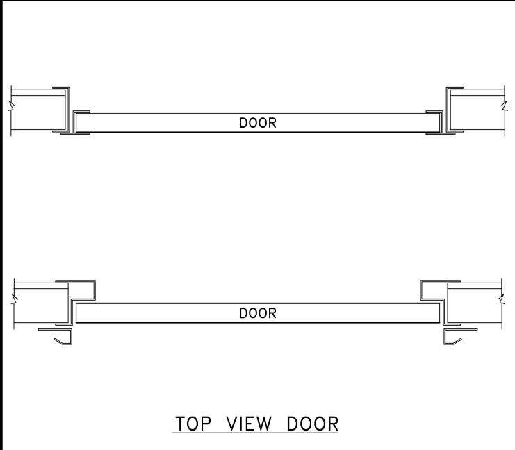
4 DETAILS FOR STEPS 2 AND 3
