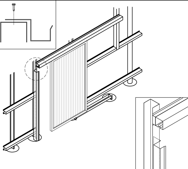
4 ATTACH DOOR TRACK STOP
