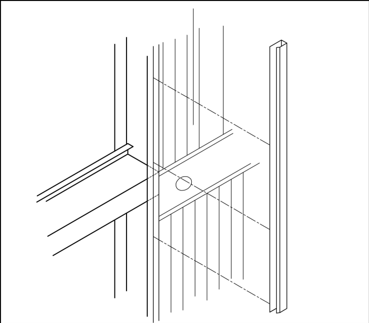
3 ATTACH FLASHING
