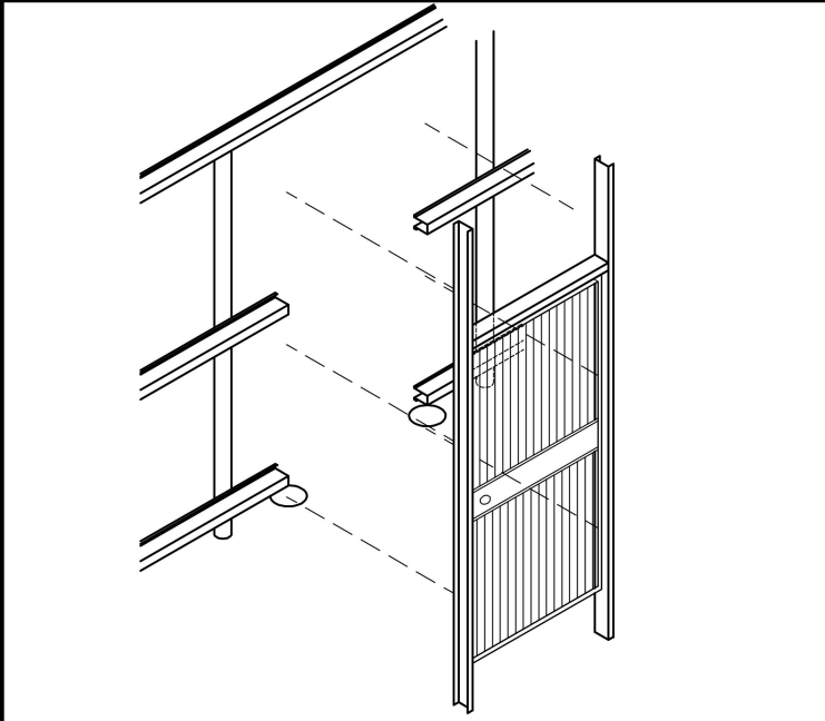
2 ASSEMBLING SWING DOOR
